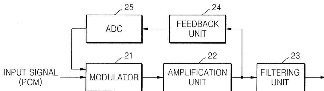
FIG. 2 (RELATED ART)
