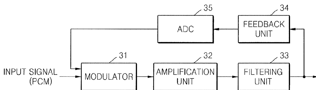
FIG. 3 (RELATED ART)
