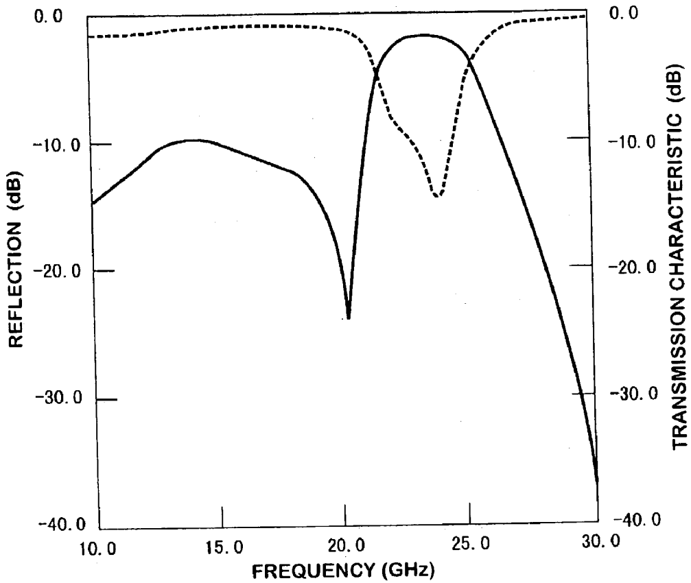
Fig. 13 PRIOR ART
