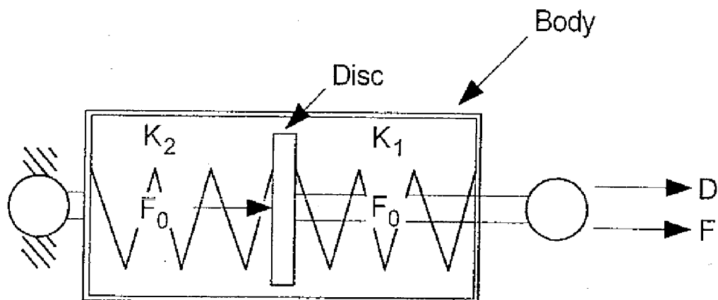
Free-body diagram
