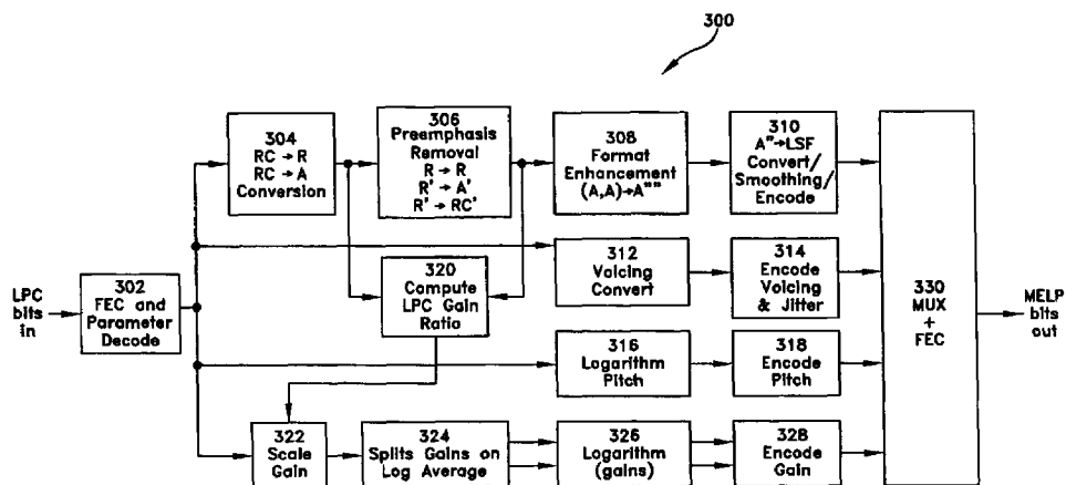
LPC to MELP Transcoder
