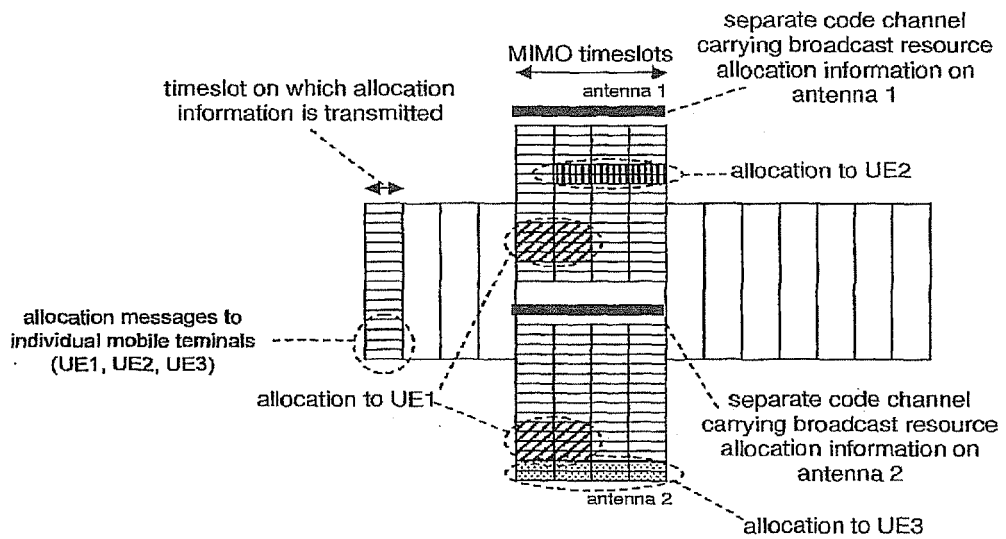
Transmission of broadcast resource allocation information via a separate code channel
