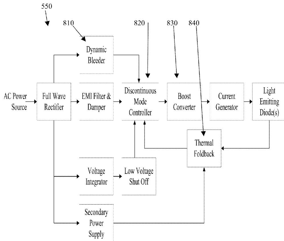
FIG. 4 Electrical Block Diagram
