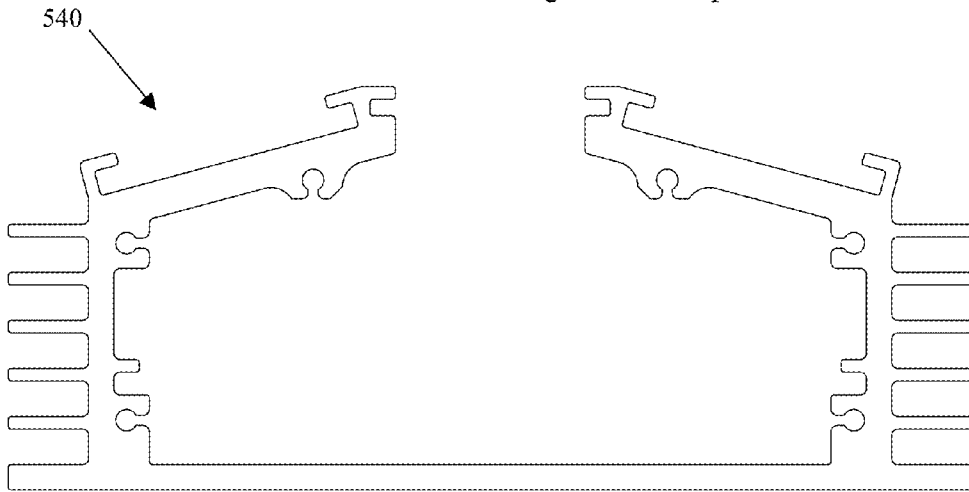
FIG. 2A Extrusion design as used in production
