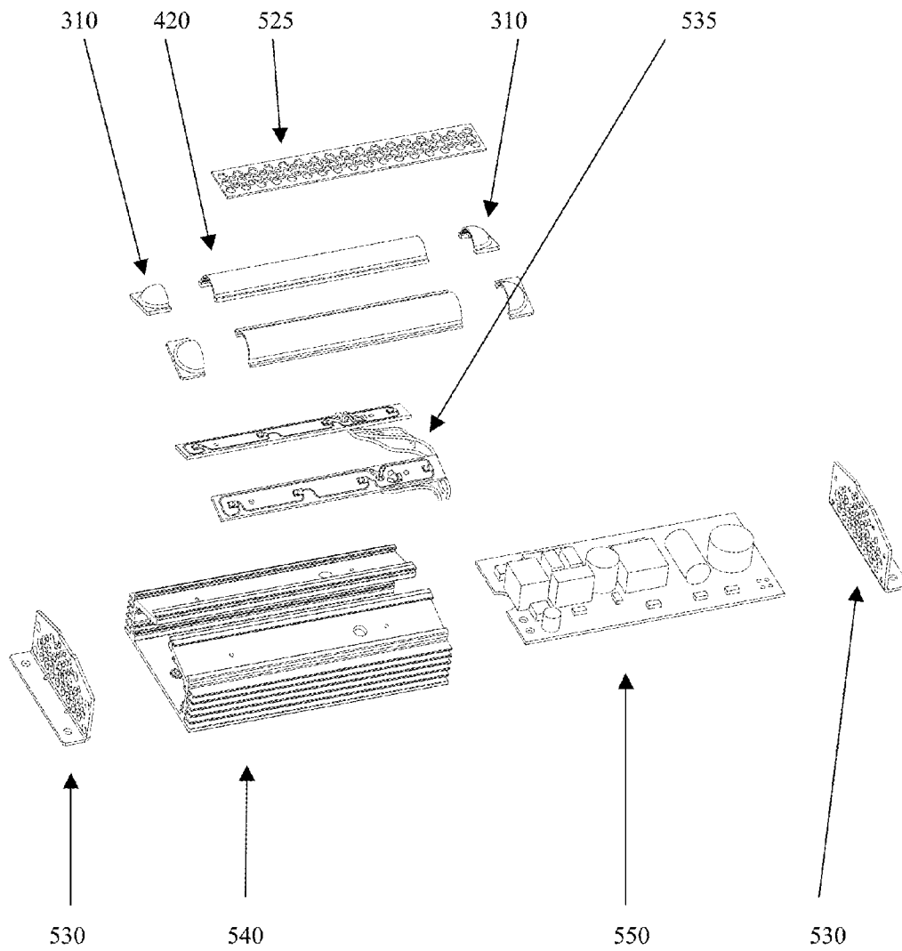
FIG. 1B Exploded Assembly
