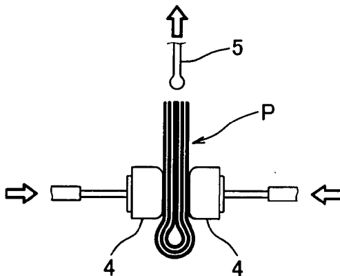
FIG. 4C PRIOR ART
