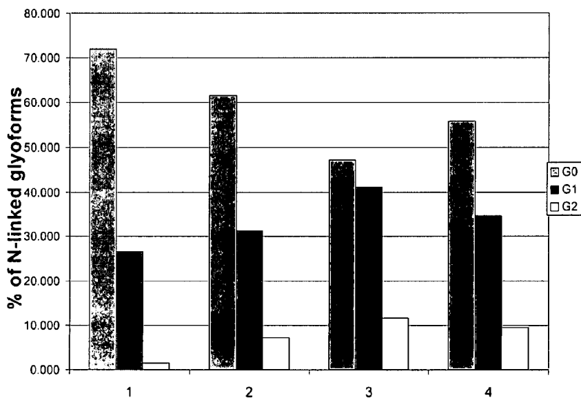
Figure 8. Graphical Comparison of Percentage of Total Peak Area for G0, G1, and G2 HPAEC-PED Peaks.
