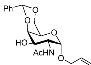
Compound 4
