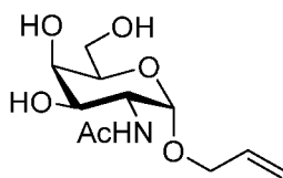
Allyl Tn
