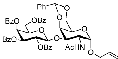
Compound 6
