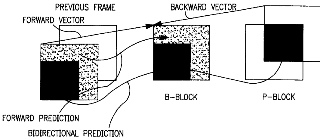
B-BLOCK PREDICTION
