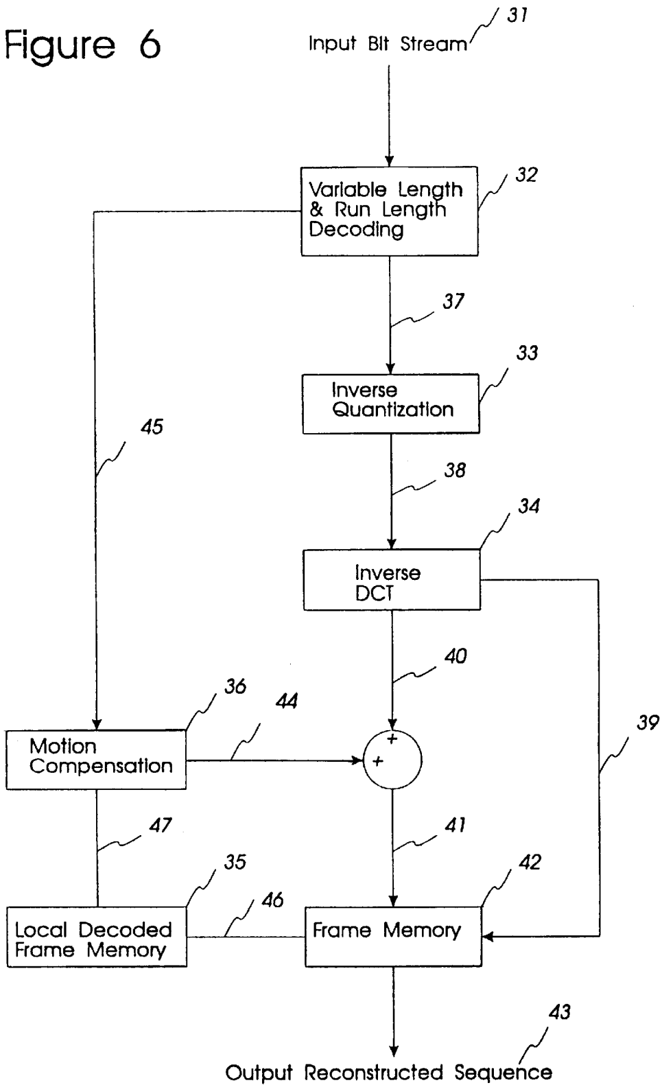
Decoder Block Diagram
