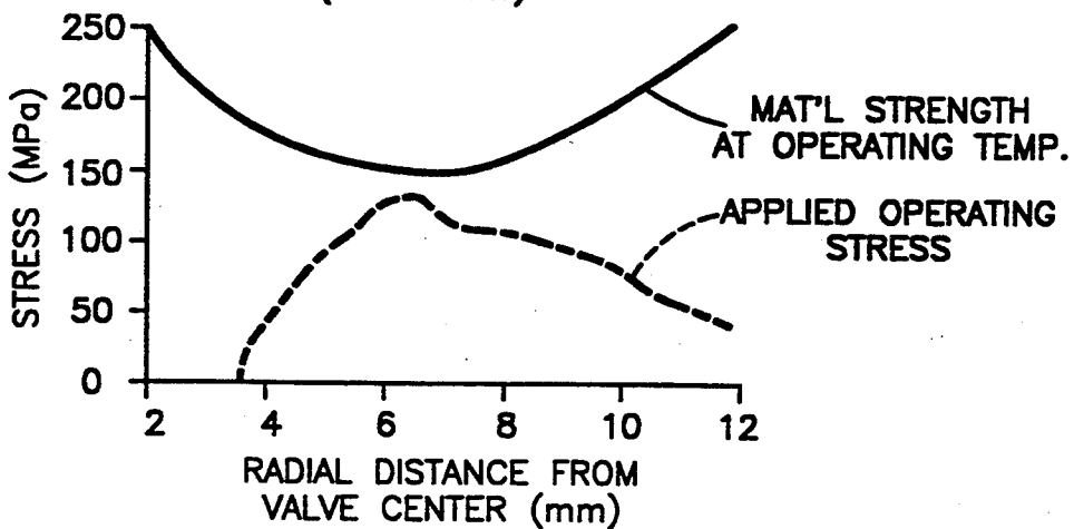
Fig.6C (PRIOR ART)
