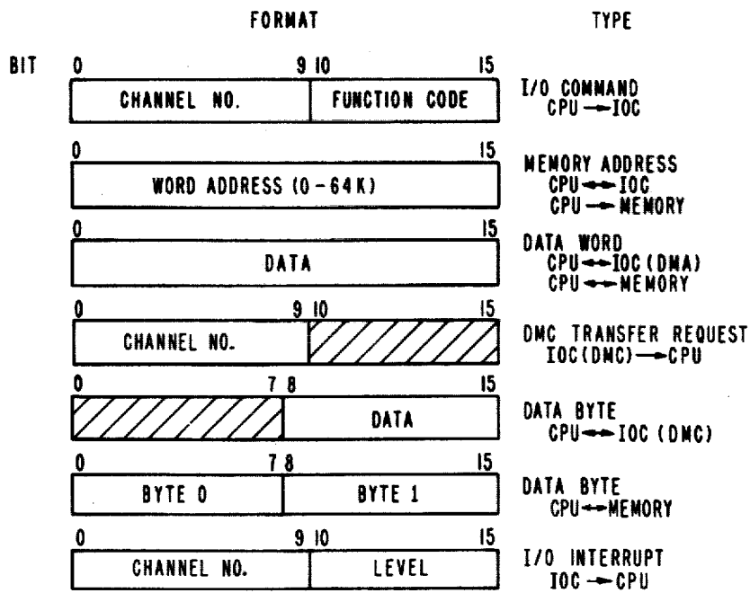
SYSTEM BUS ADDRESS / DATA LINE FORMATS
