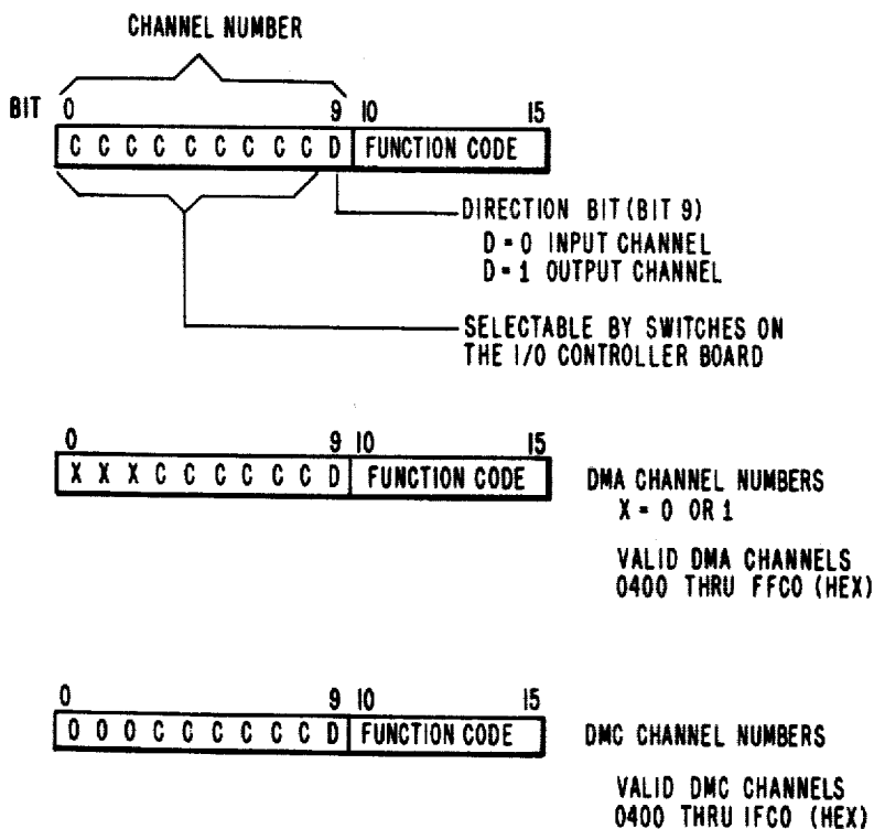
I/O SOFTWARE INSTRUCTION CONTROL WORD FORMAT
