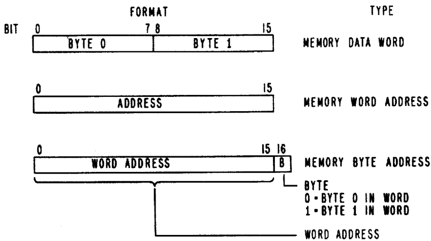
WORD AND ADDRESS FORMATS
