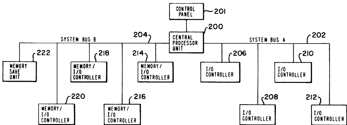
SYSTEM CONFIGURATION
