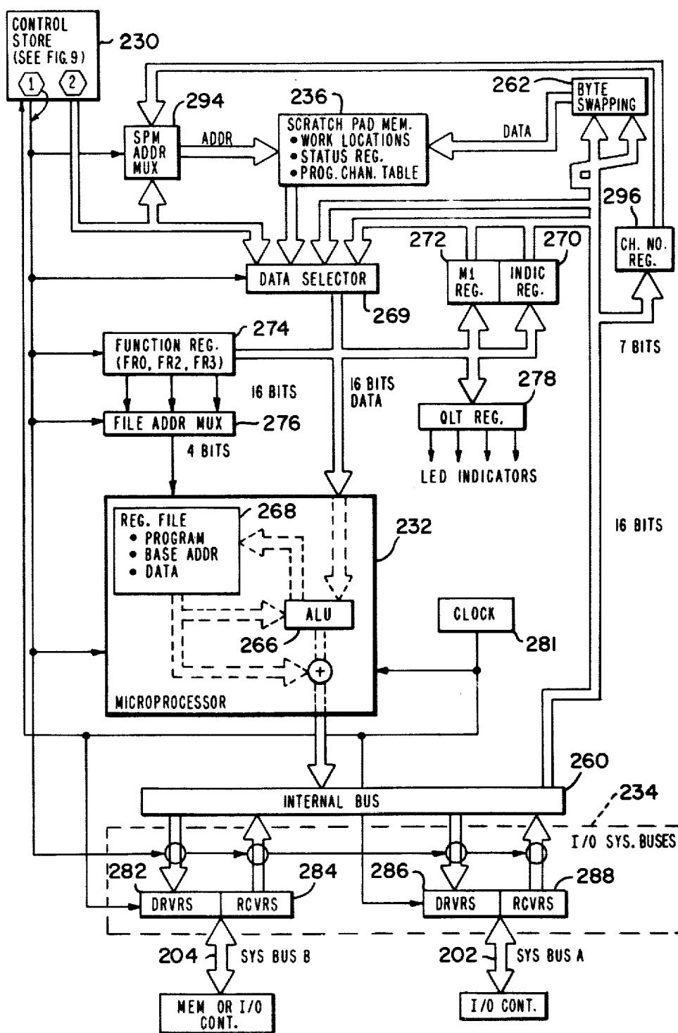
FIG. 8 CPU BLOCK DIAGRAM
