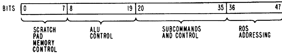
CPU FIRMWARE MICROINSTRUCTION WORD
