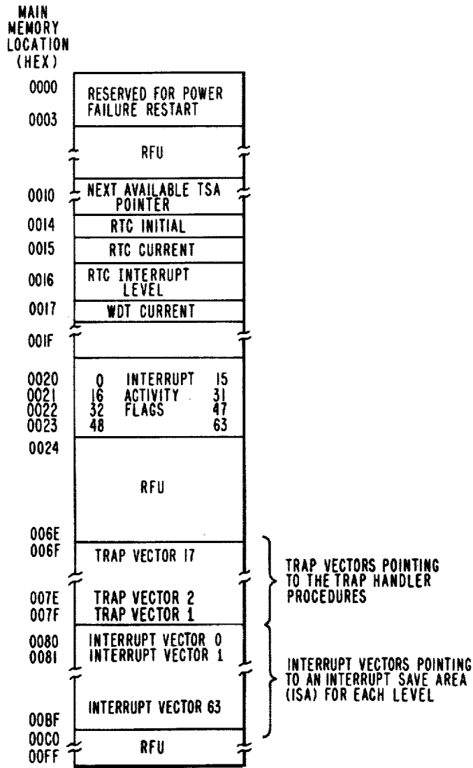
DEDICATED MAIN MEMORY LOCATIONS
