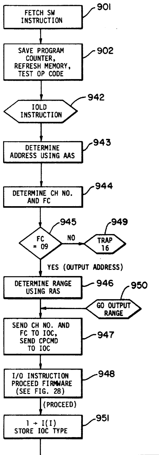
I/O INSTRUCTION FLOW CHART
