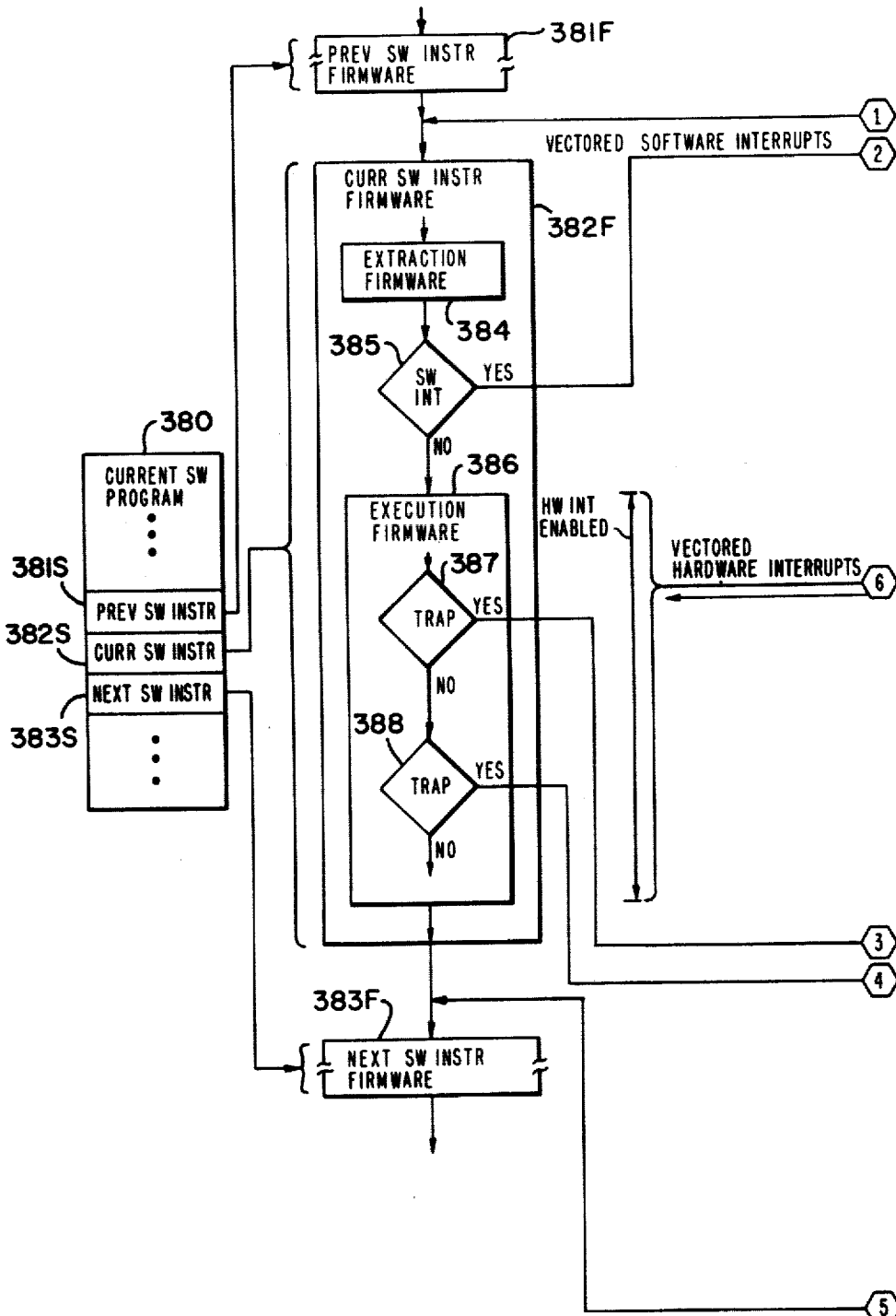
SOFTWARE INTERRUPT-TRAP-HARDWARE INTERRUPT INTERACTION FIG. 34 SHEET 1 OF 2
