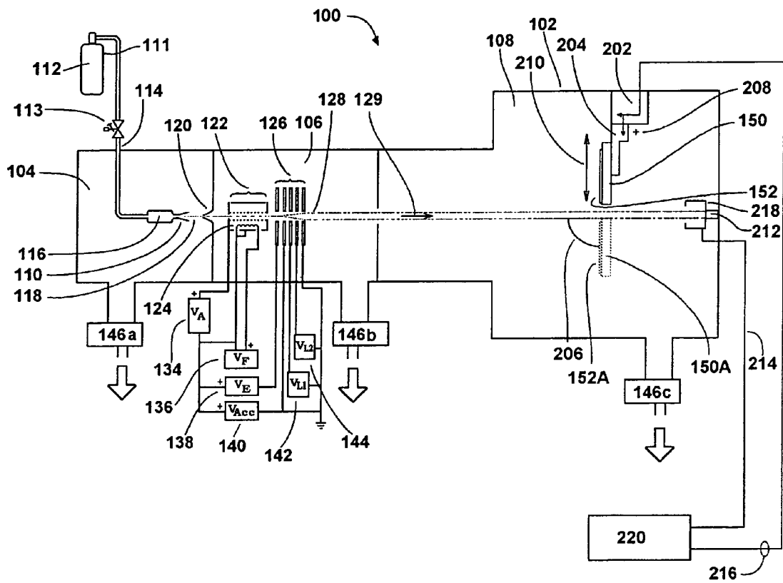
Figure 1 Prior Art.
