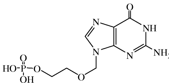
Acyclovir monophosphate
