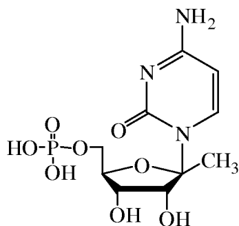
2'-C-methyl-cytidine-5'-phosphate
