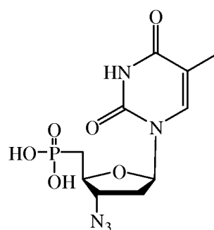
AZT 5'-phosphonate
