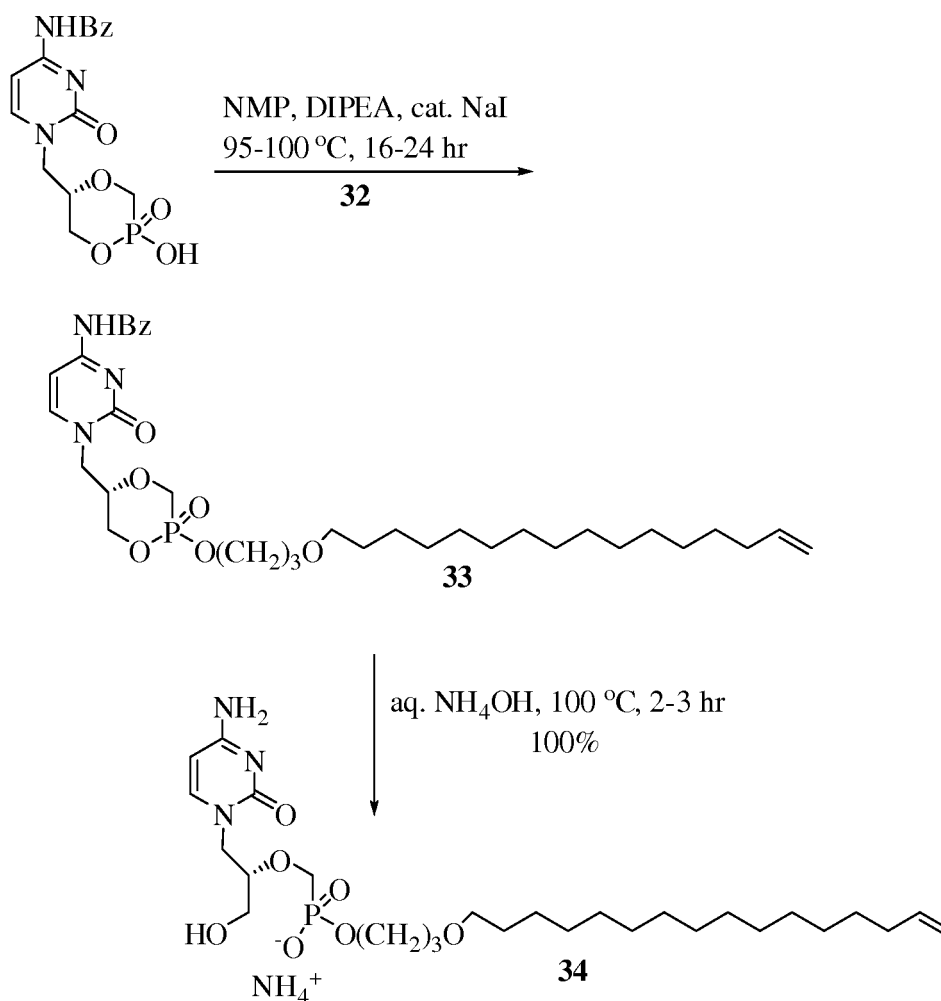
Scheme 5
