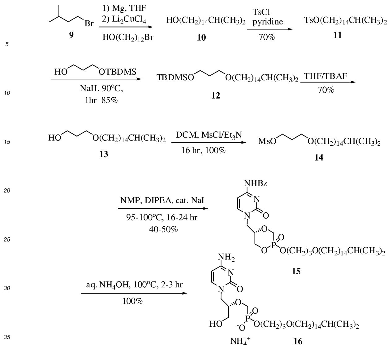
Scheme 3
