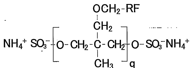
Structural Formula (3)
