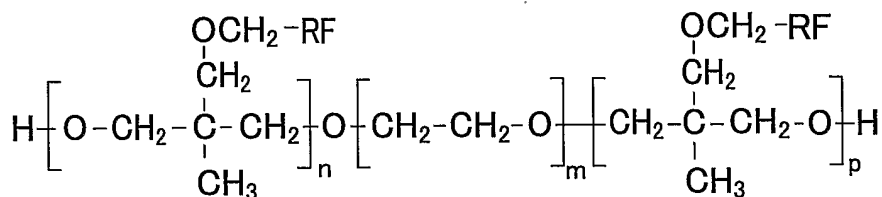
Structural Formula (2)
