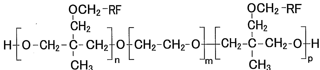
Structural Formula (2)
