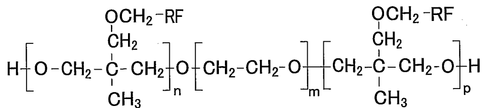
Structural Formula (2)
