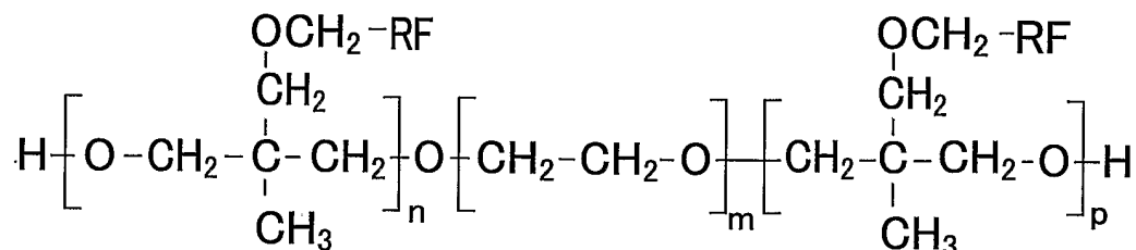
Structural Formula (2)
