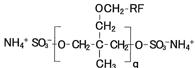
Structural Formula (3)
