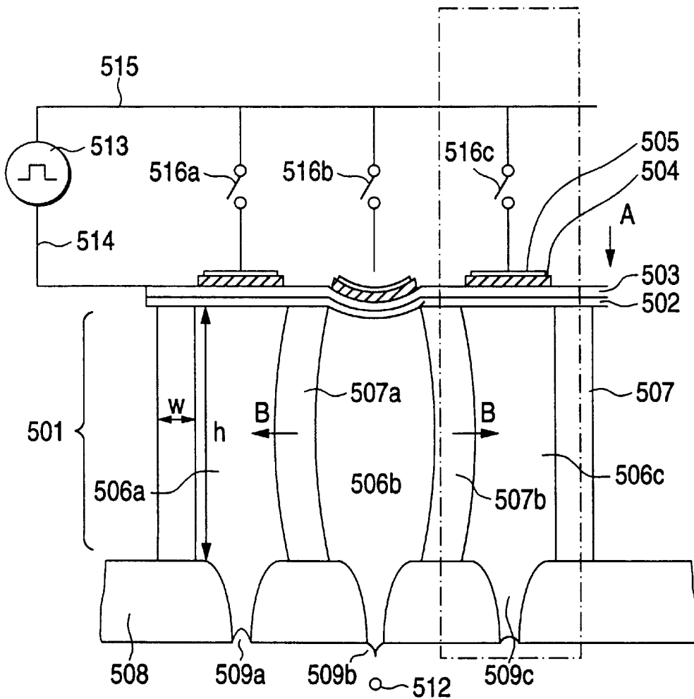
FIG. 21 CONVENTIONAL ART
