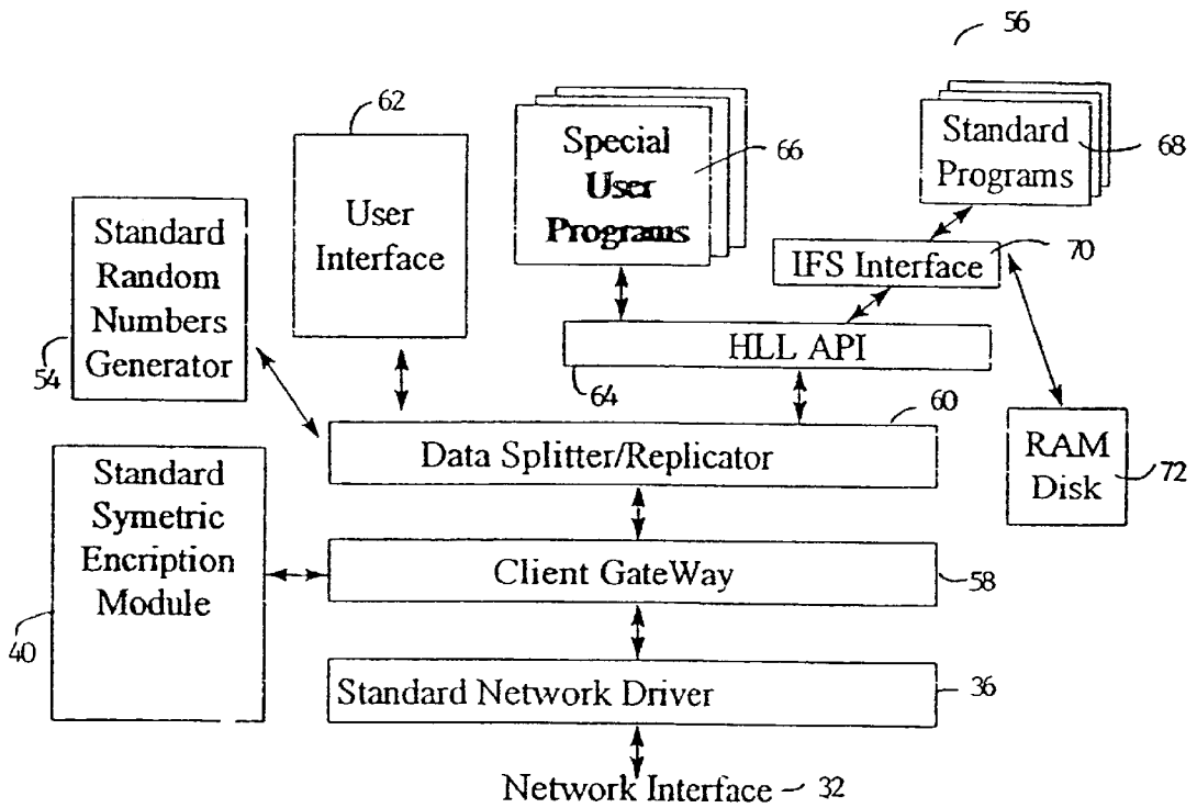
BLOCK DIAGRAM OF CLIENT
