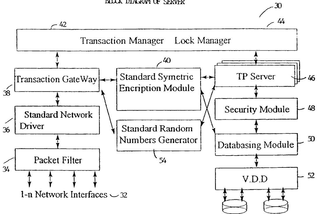
BLOCK DIAGRAM OF SERVER
