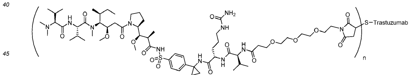
T-MT-Compound 5
