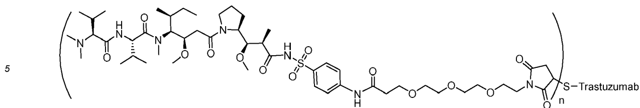
T-MCvcPABC-Compound 80
