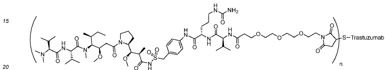
T-MTvc-Compound 32
