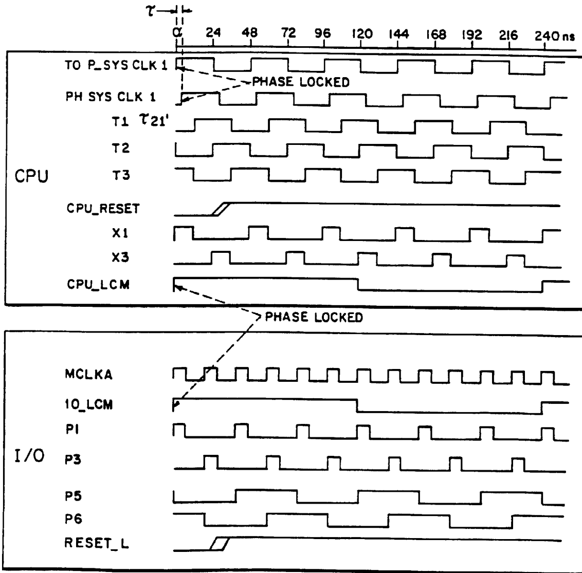
(CLOCK TIMING DIAGRAMS)
