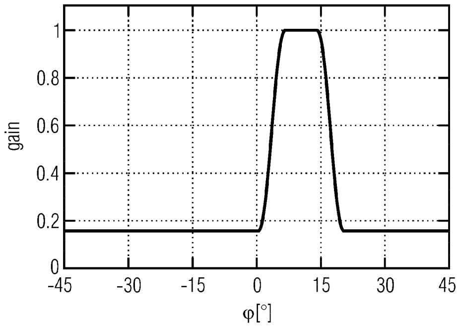
window function after zooming with a shift
