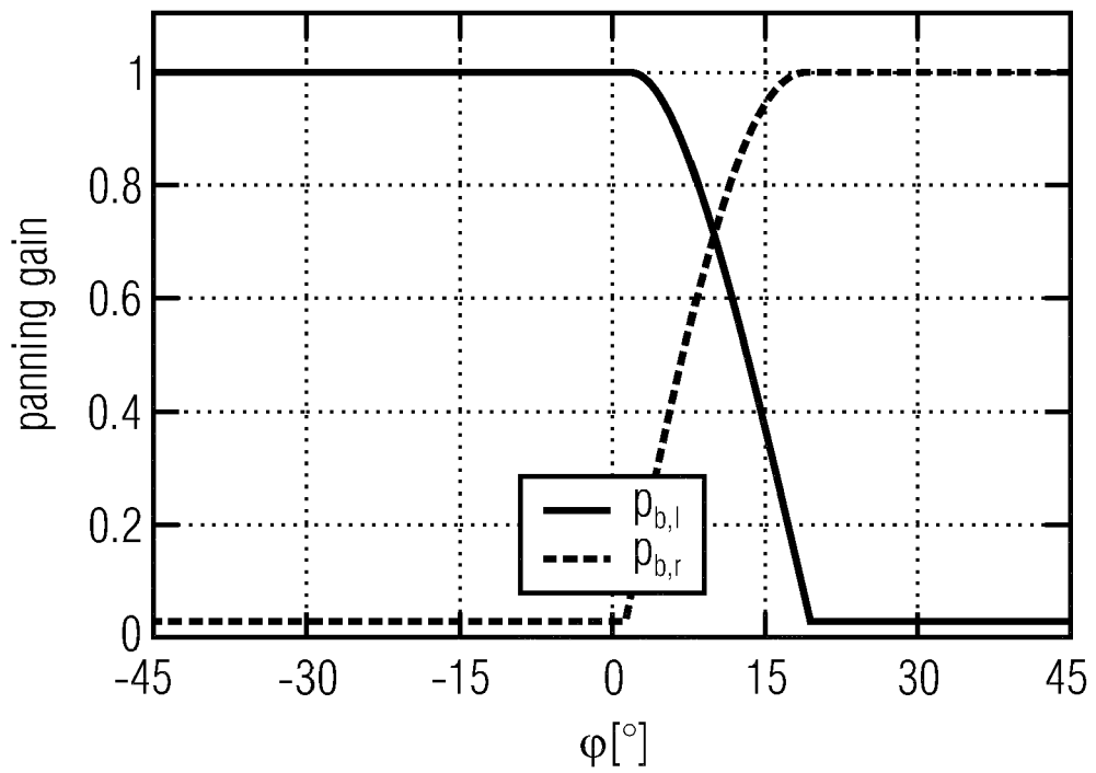
panning function after zooming with a shift
