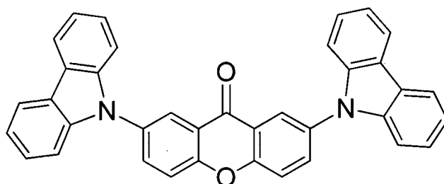
Compound 1
