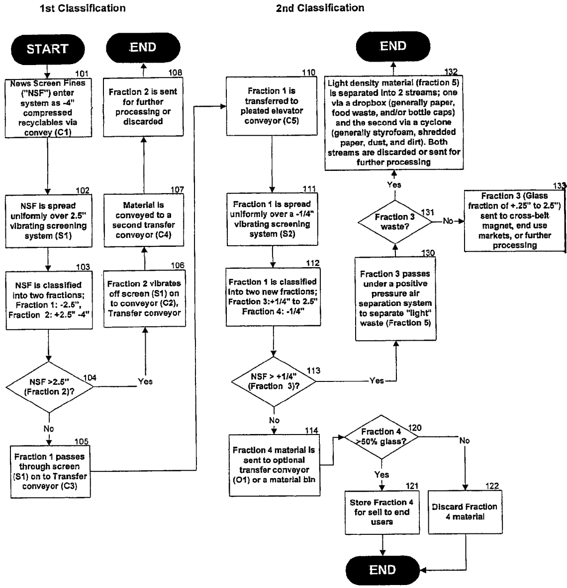
News Screen Fines System Flow Diagram
