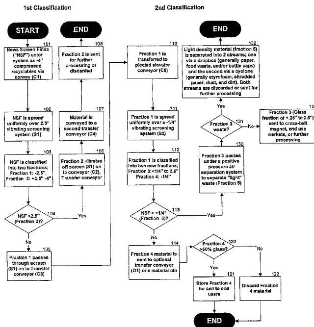
News Screen Fines System Flow Diagram
