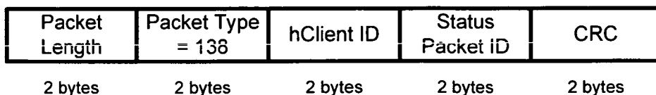
Figure, Request Specific Status Packet
