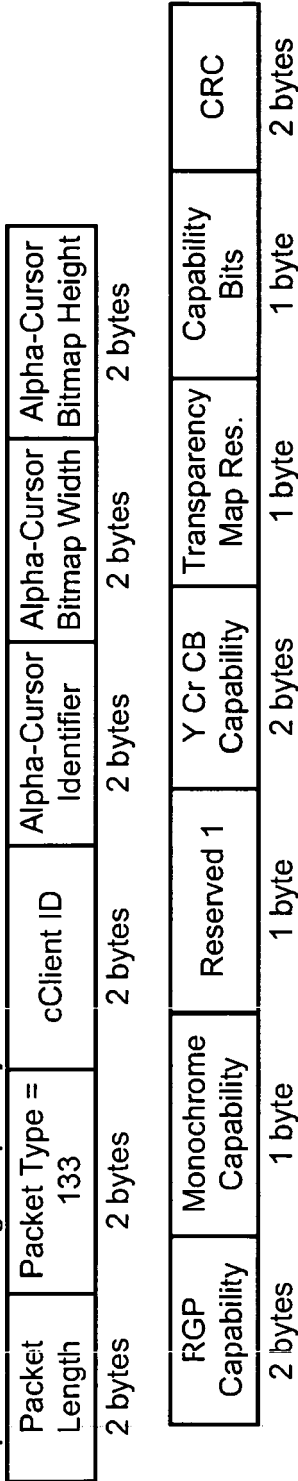
Alpha-Cursor Image Capability Packet
