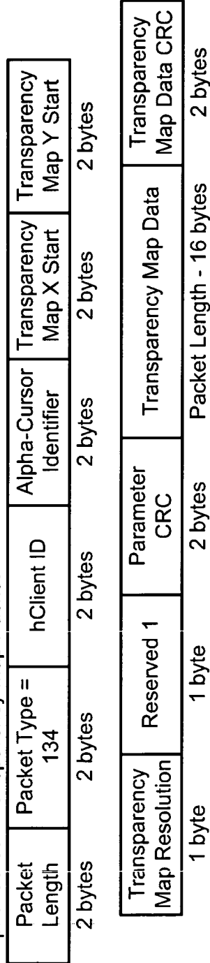
Alpha-Cursor Transparency Map Packet
