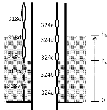
(c) Case 2 SSS inlet riser discharge
