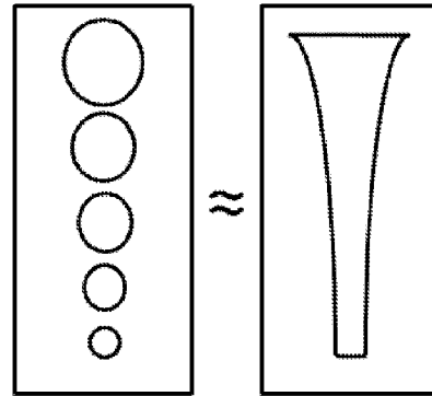
(a) Skimmer first riser equivalent weir
