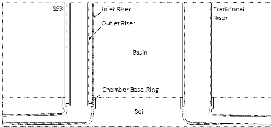
(a) Skimmer risers installed in basin
