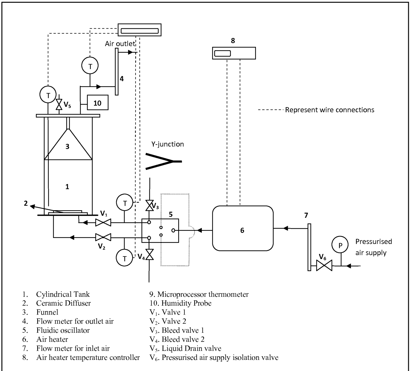
Figure 1: Equipment Set-Up
