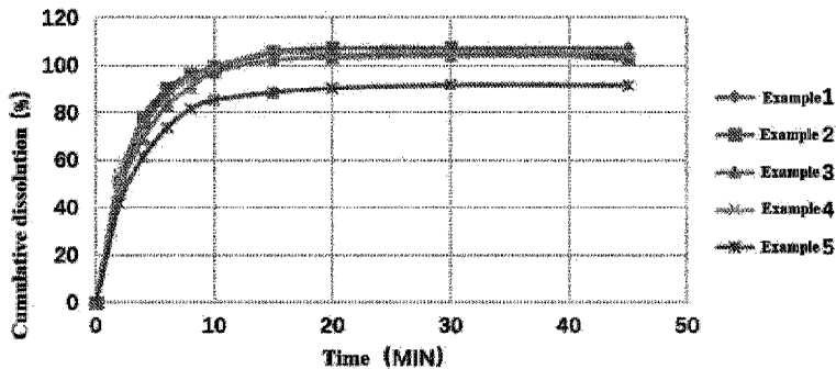
Dissolution profile
