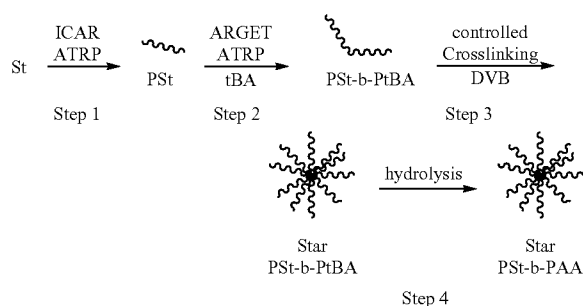
Scheme 3. Multistep synthesis of PST-b-PAA block copolymer stars
