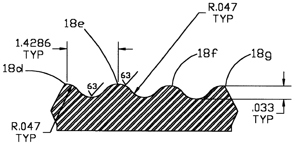
DETAIL A
