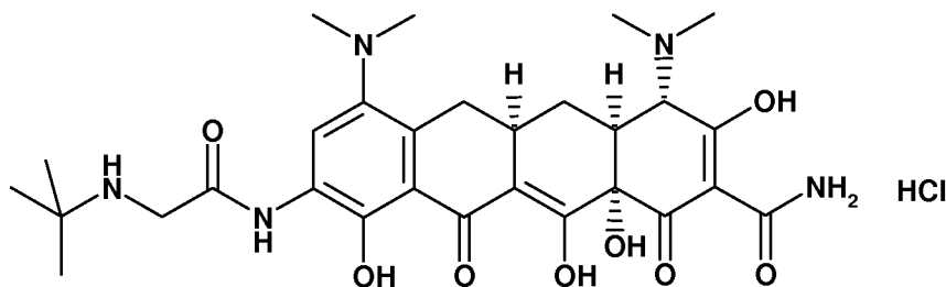
35 Figure A: Chemical structure of Tigecycline hydrochloride
