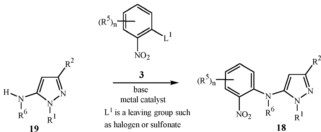
Scheme 10
