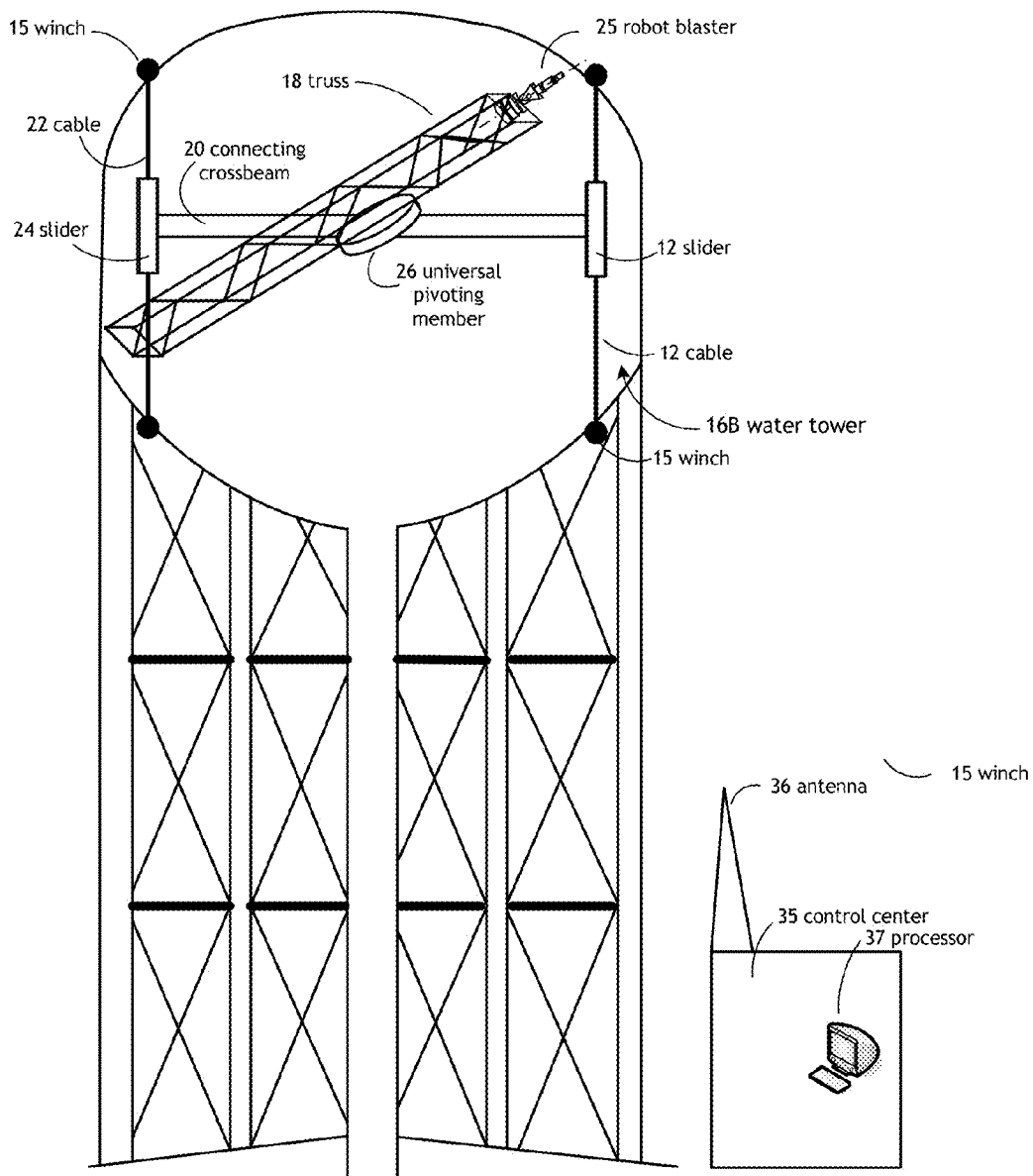
FIGURE 1B SURFACE MEDIA BLASTER
