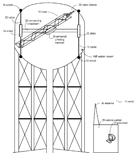
SURFACE MEDIA BLASTER
