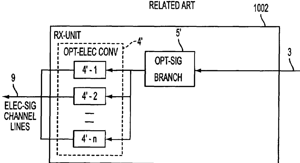
FIG. 1C RELATED ART
