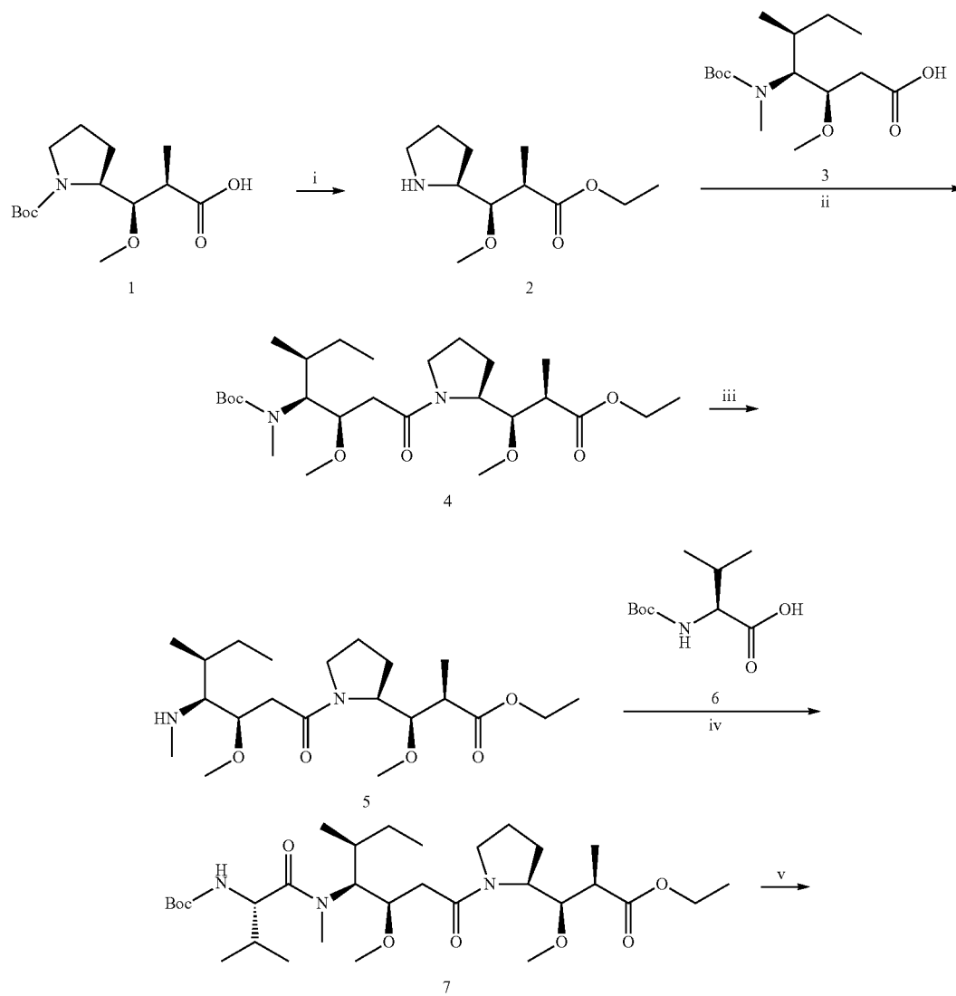
SCHEME I
