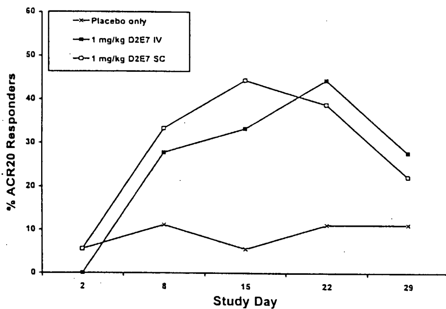
Percentage of ACR20 responders following a single i.v. injection of D2E7 and/or placebo (DE010)
