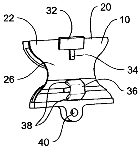
FIG. 3 (Prior Art)
