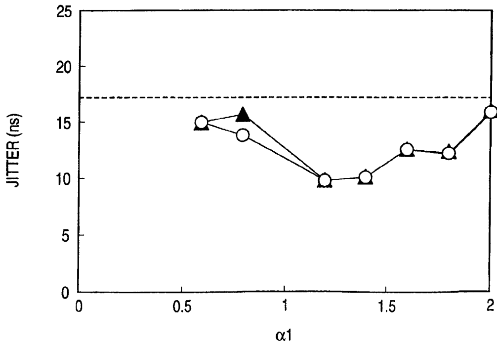
MARK AND SPACE JITTER
