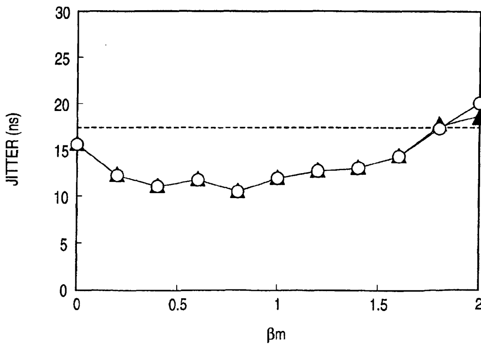
MARK AND SPACE JITTER
