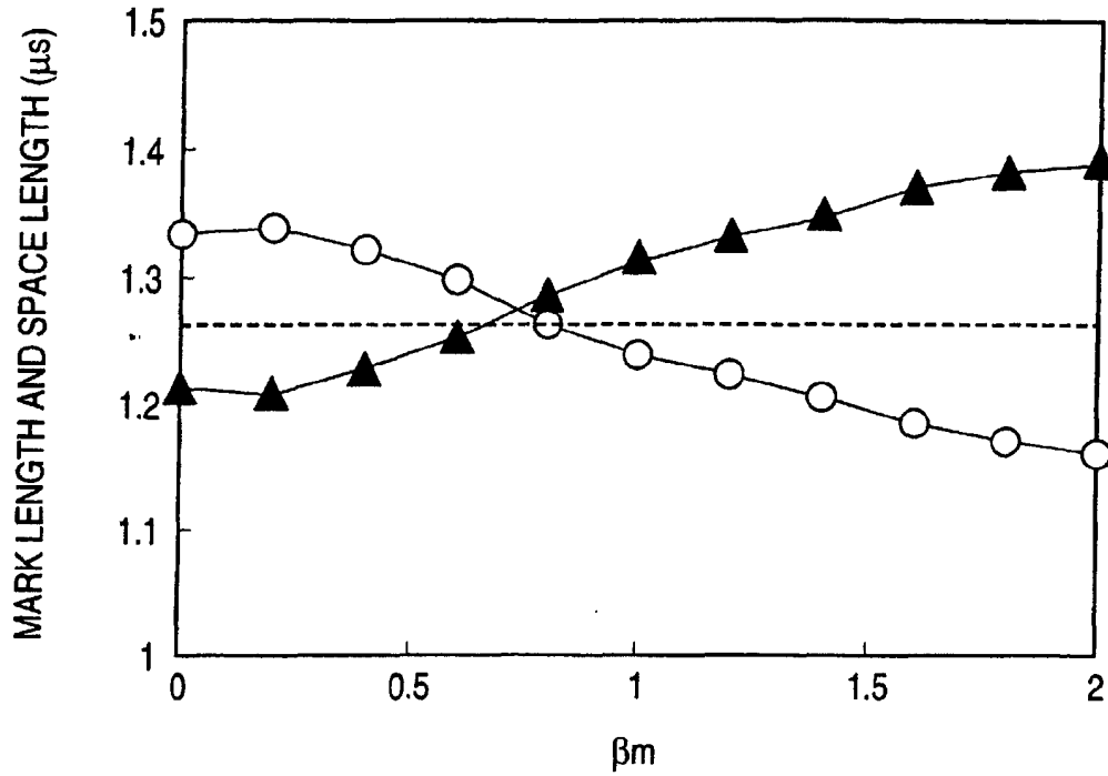
MARK LENGTH AND SPACE LENGTH
