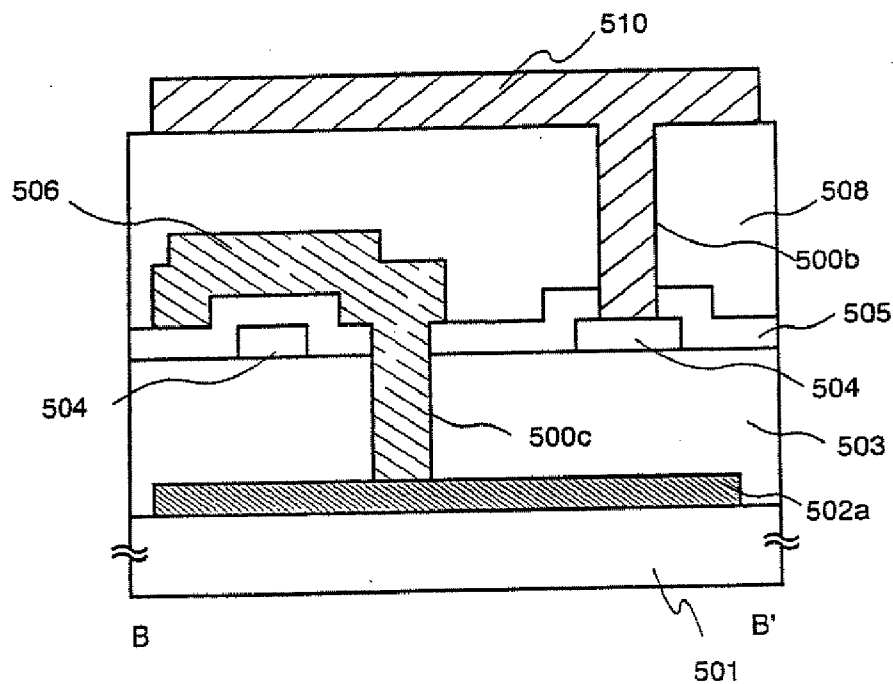
Fig. 15B B-B' Cross sectional view
