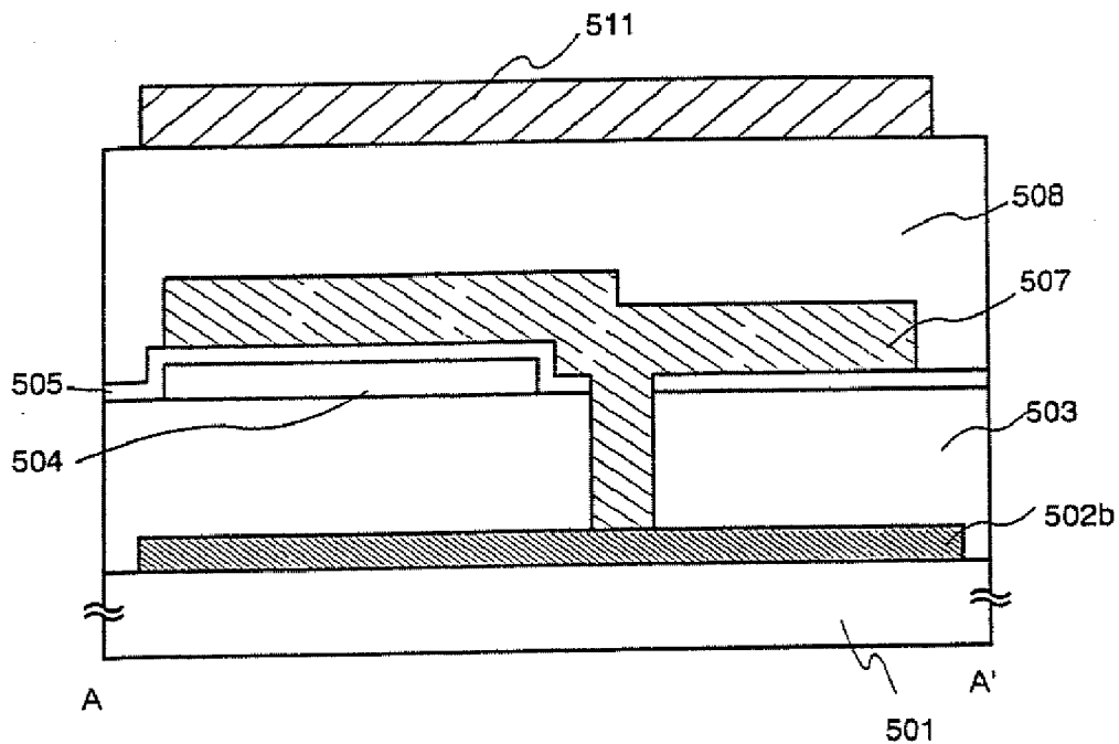
Fig. 15A A-A' Cross sectional view
