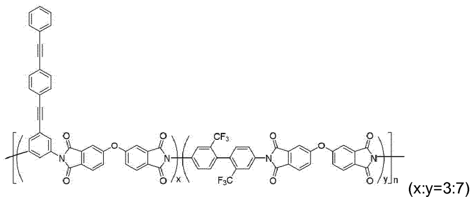
Chemical Formula C-4
