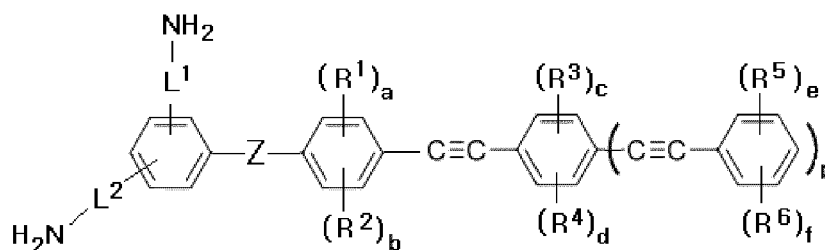
Chemical Formula 1-1b
