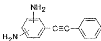
Chemical Formula 1d
