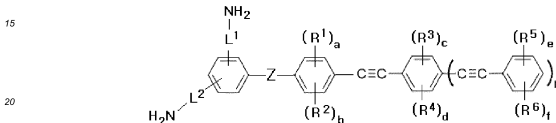
Chemical Formula 1-1b
