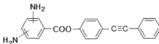
Chemical Formula 1d
