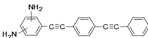
Chemical Formula 1a
