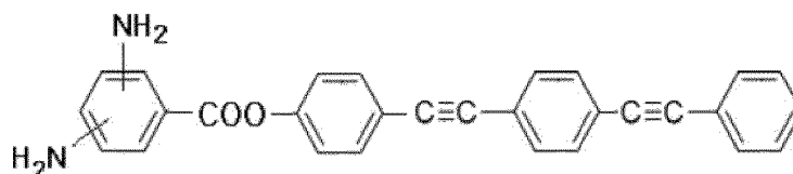
Chemical Formula 1c
