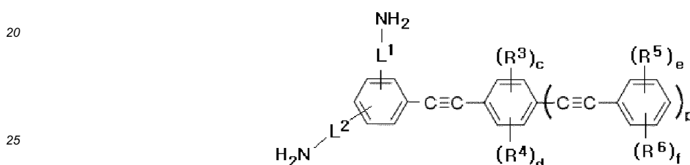
Chemical Formula 1-1a
