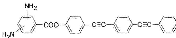
Chemical Formula 1b
