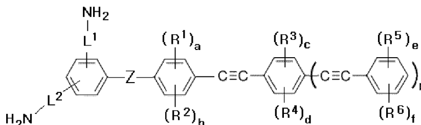
30 Chemical Formula 1-2b
