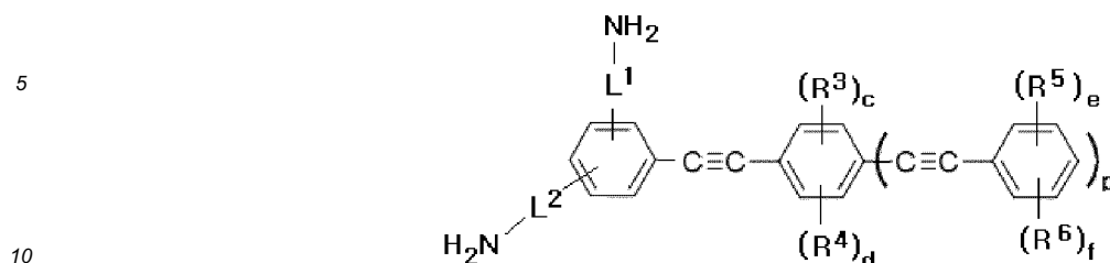
Chemical Formula 1-1b
