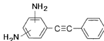
Chemical Formula 1c
