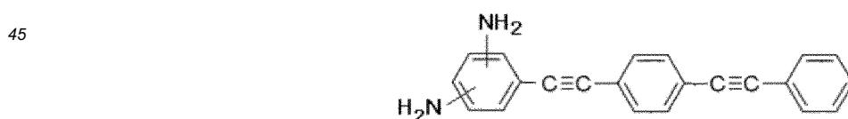
Chemical Formula 1a
