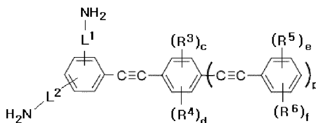
30 Chemical Formula 1-2b
