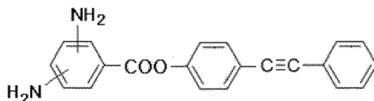
Chemical Formula 1d
