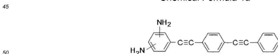
Chemical Formula 1a
