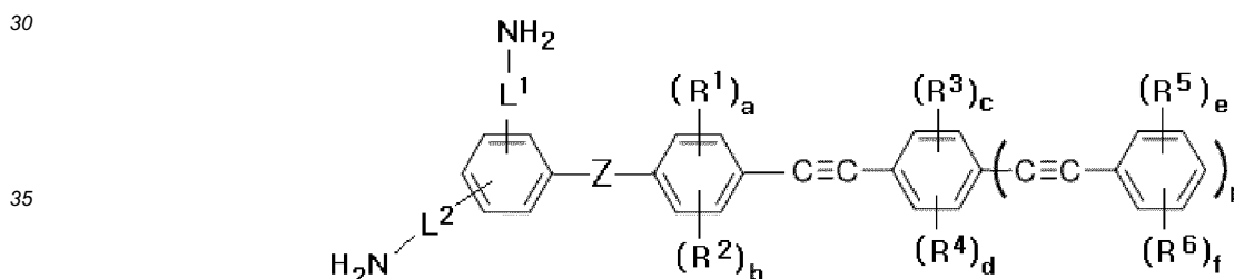
Chemical Formula 1-1b
