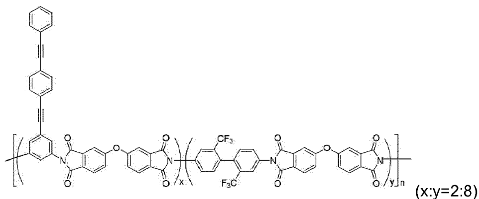
Chemical Formula C-3
