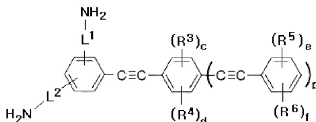
Chemical Formula 1-1b
