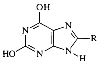
R=H=Xanthine R=OH=Uric Acid
