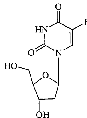
Floxuridine
