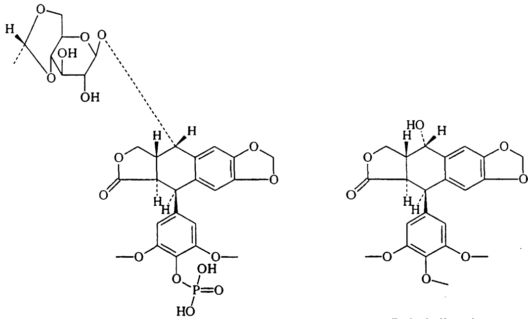
Podophyllotoxin
