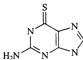
6-Thioguanine
