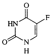
Fluorouracil (5-FU)
