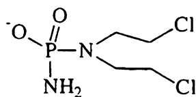
Phosphoramidate Mustard
