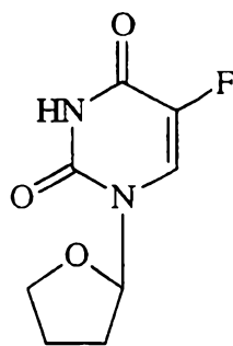
Ftorafur
