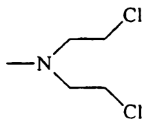
Mechlorethamine
