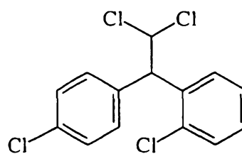
Mitotane
