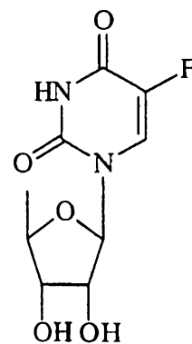
5'-deoxyfluorouridin
