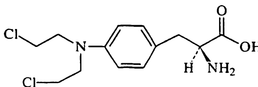
Melphalan
