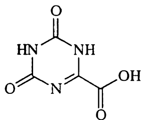
Oxonic Acid
