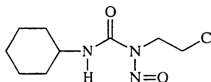
Lomustine (CCNU)
