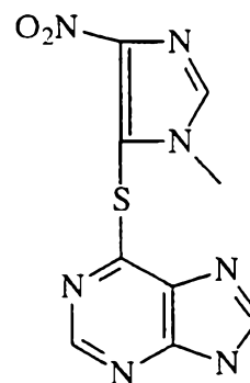
Azathioprine
