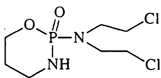
Cyclophosphamide
