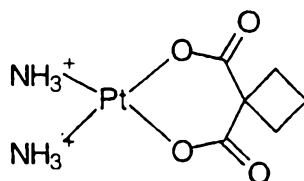
Carboplatin
