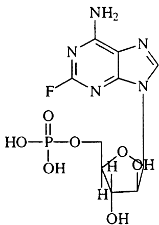
Fludarabine Phosphate
