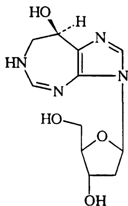
Pentostatin
