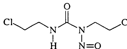
Carmustine (BCNU)
