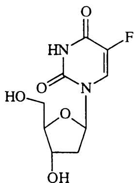
Floxuridine
