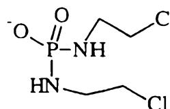
Isophosphoramidate Mustard
