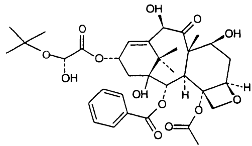
Taxotere
