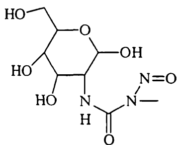
Streptozocin
