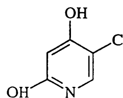
CDHP
