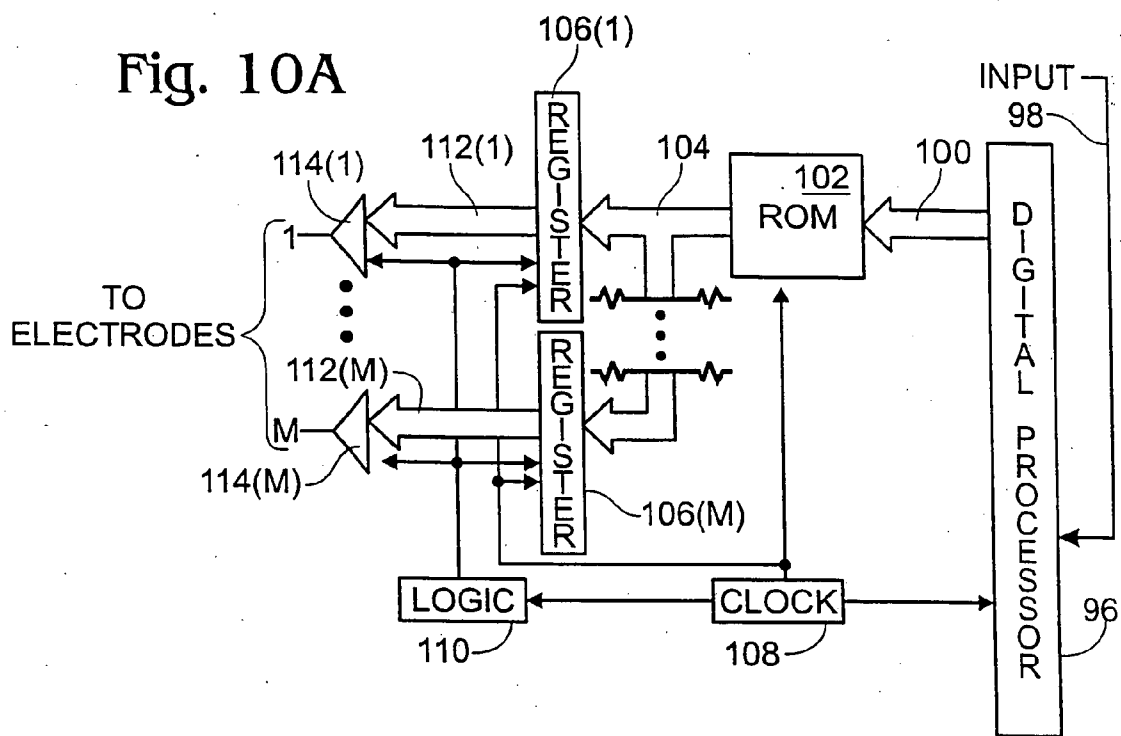
TO ELECTRODES
