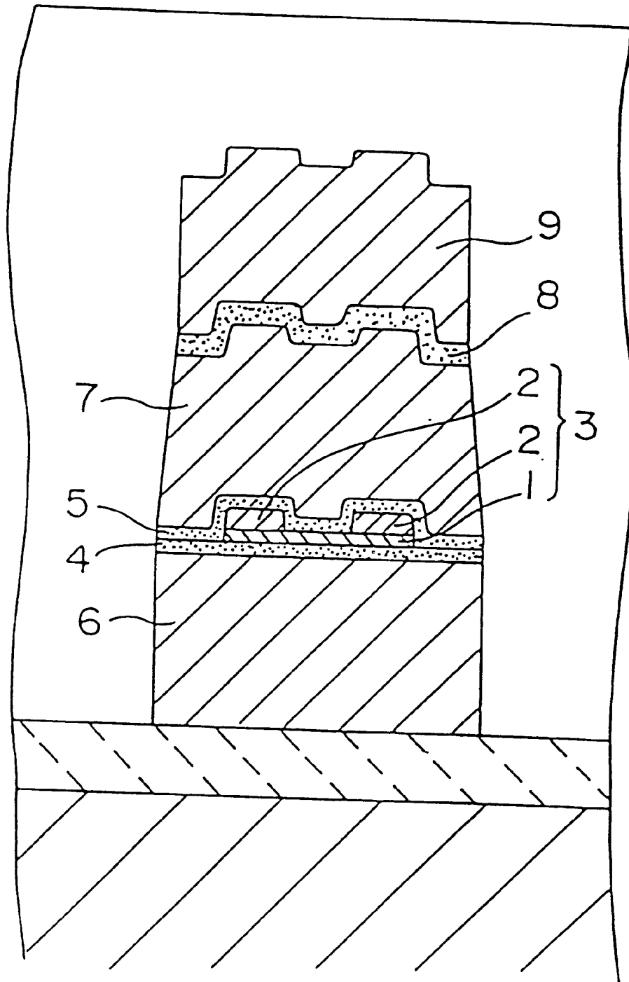
FIG. 27 PRIOR ART
