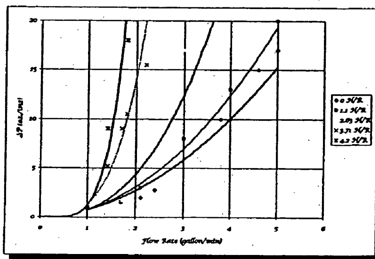
Figure 32: Relationship of Flow Rate and \Delta P in the Composite of Several Coating Weights
