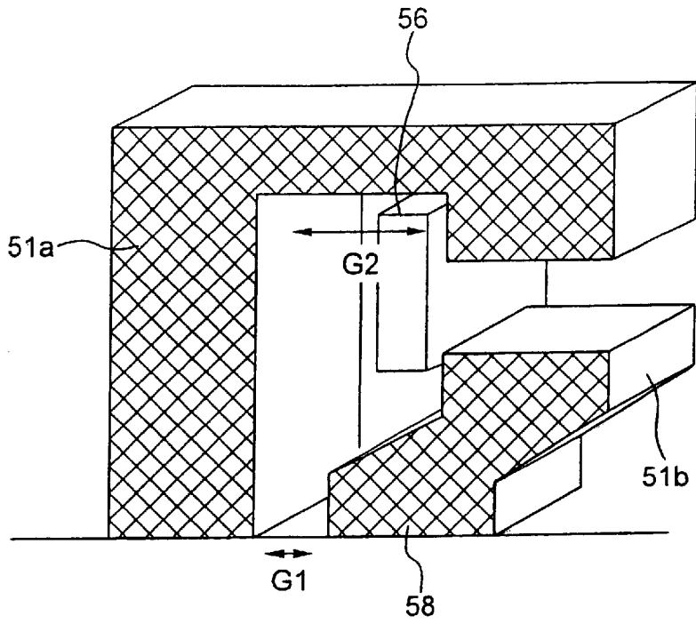
FIG. 19 PRIOR ART
