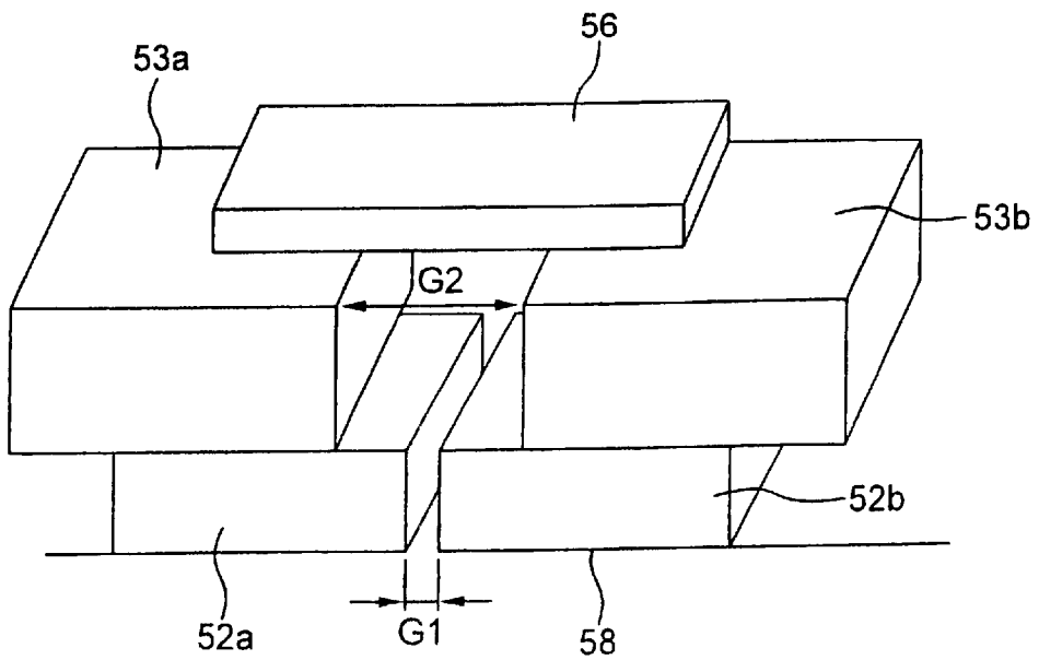
FIG. 20 PRIOR ART
