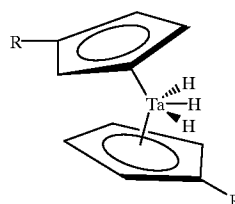
III Bis(cyclopentadienyl) tantalum (V) trihydride
