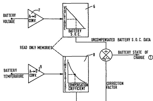
BATTERY S.O.C. MEASUREMENT BY O/C VOLTAGE INSPECTION
