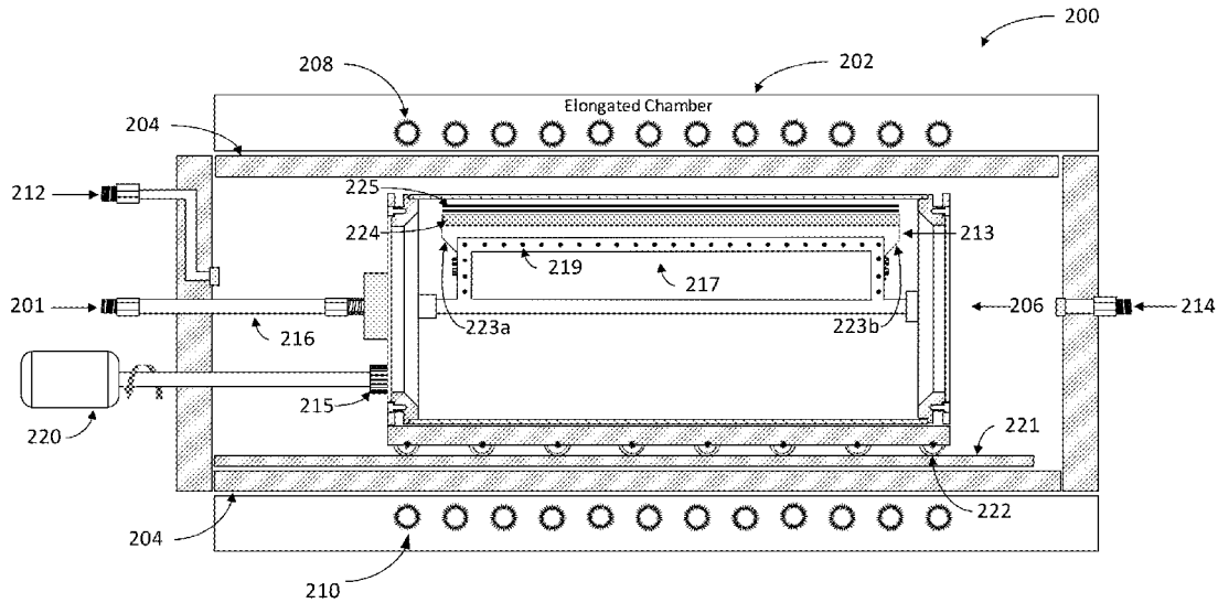
Low-pressure CVD (LPCVD) system
