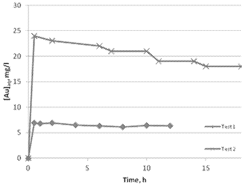
Figure 9. Gold concentrations vs. leaching time in tests 1 and 2 of Example 3. Test 1: [Cu^{2+}]_{aq,0}=100 g/l, [NaBr]_{aq,0}=100 g/l, [Cl^-]_{aq,0}=225 g/l, [solid]_0=50 g/l, pH=1.7 , T=98^{\circ}C , oxygen feed 1.5 l/min, and material from POX test 1. Test 2: [Cu^{2+}]_{aq,0}=20 g/l, [NaBr]_{aq,0}=8-100 g/l, [Cl^-]_{aq,0}=150 g/l, [solid]_0=315 g/l, [acid]_{HCl}=10 g/l, T=98^{\circ}C , oxygen feed 2 l/min, and material from POX test 1.
