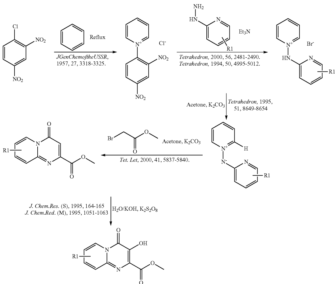
General Scheme 2: Alternate Synthesis 1
