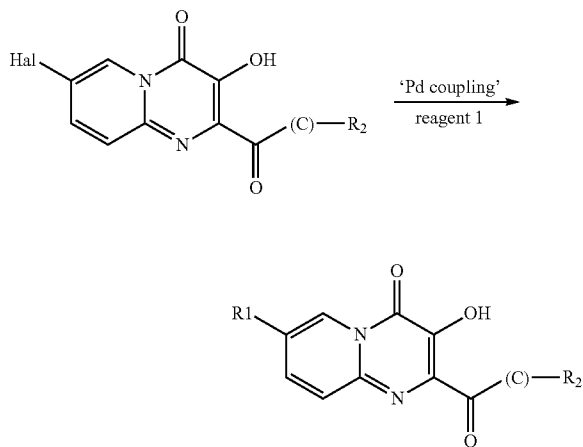
Further reactions: Scheme 4
