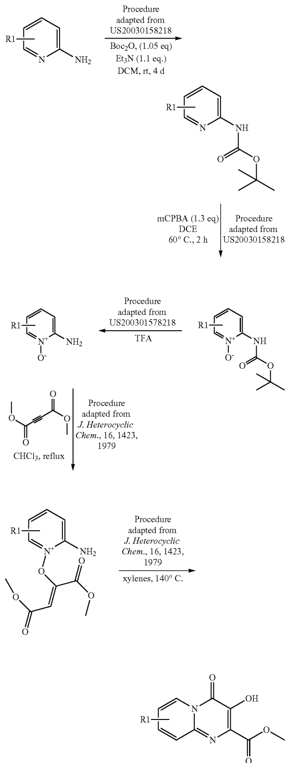
General Scheme 3: Alternate Synthesis 2
