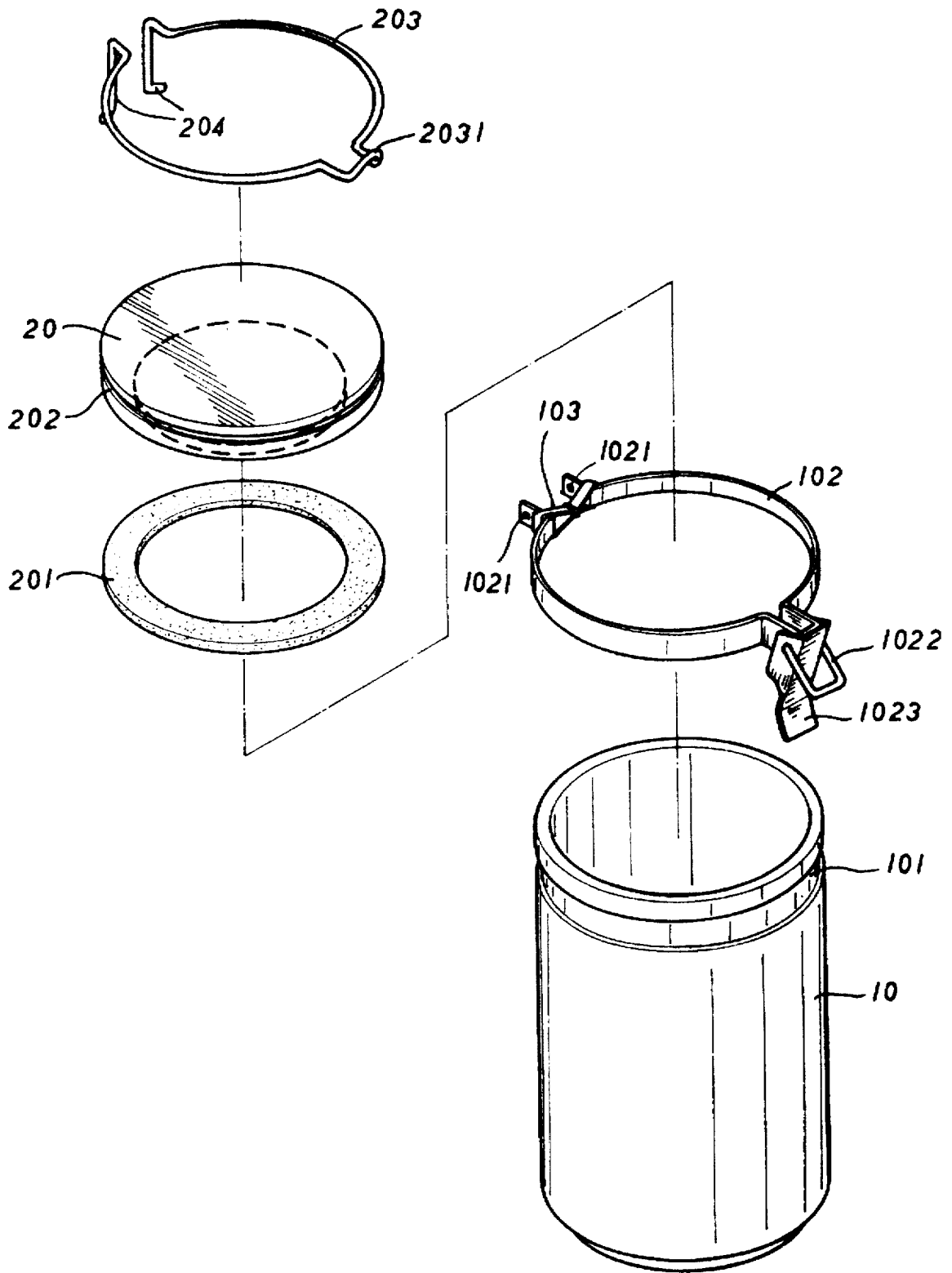
FIG. 1 (Prior Art)
