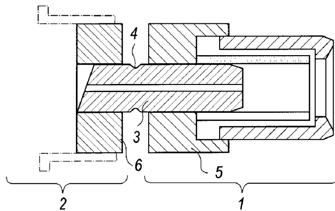
Fig. 7B (prior art)
